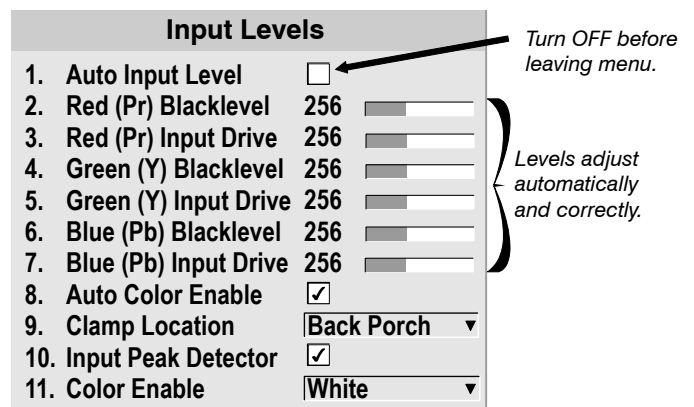
FIGURE 3-28 INPUT LEVELS
