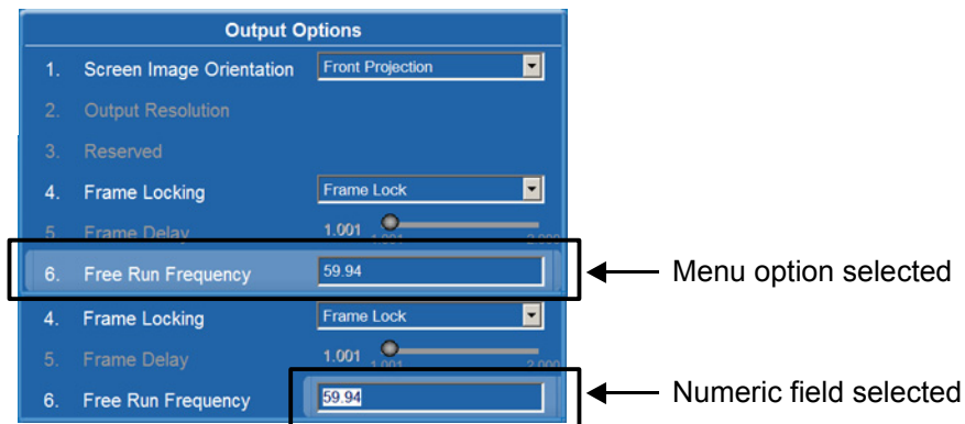
FIGURE 4-8 SELECT NUMERIC FIELD
