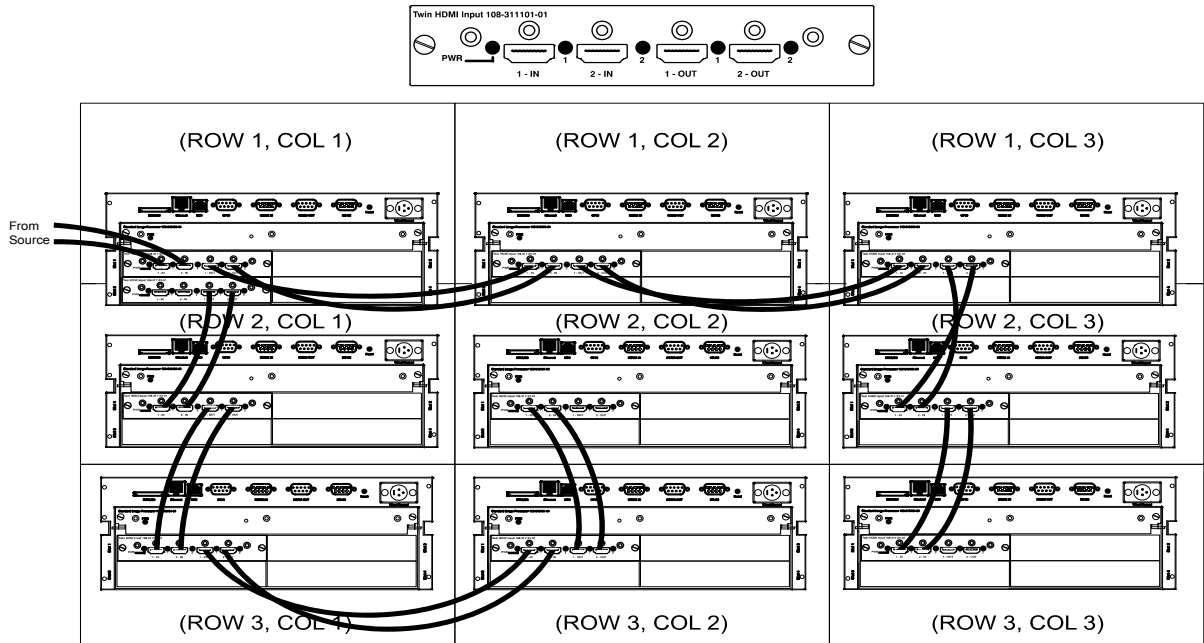
FIGURE 2-31 3X3 LOOP-THROUGH WIRING SOLUTION
