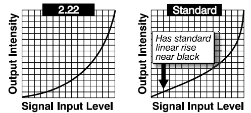
FIGURE 3-30 GAMMA CURVE
