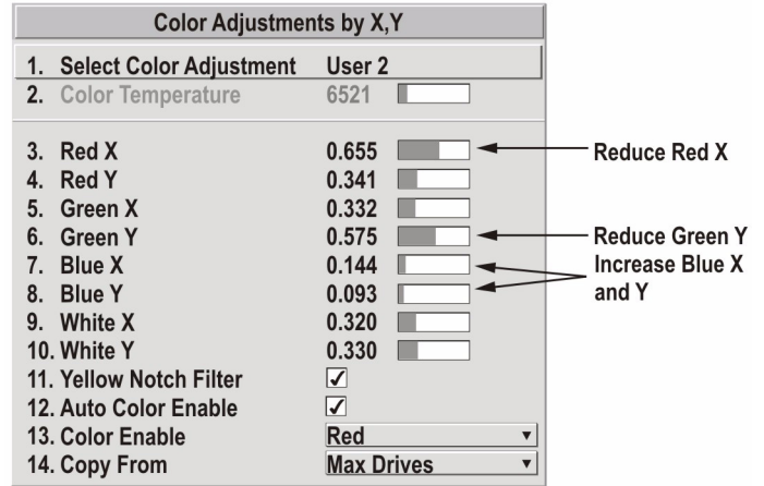
FIGURE 3-43 COLOR ADJUSTMENT
