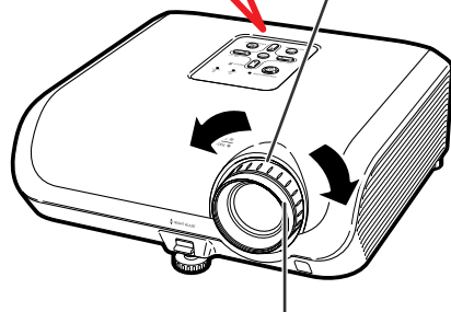
Focus ring
