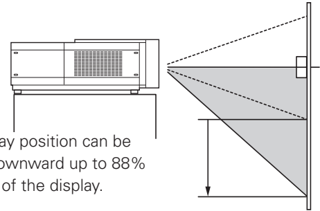
When the lens is shifted to bottom.
