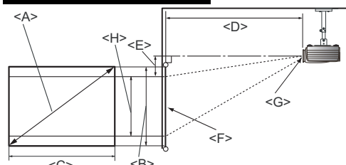
Ceiling Installation
