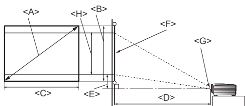
Floor Installation
