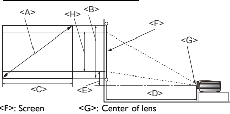
Floor Installation
