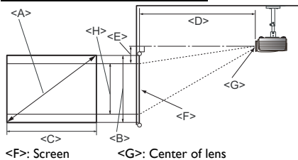
Ceiling Installation
