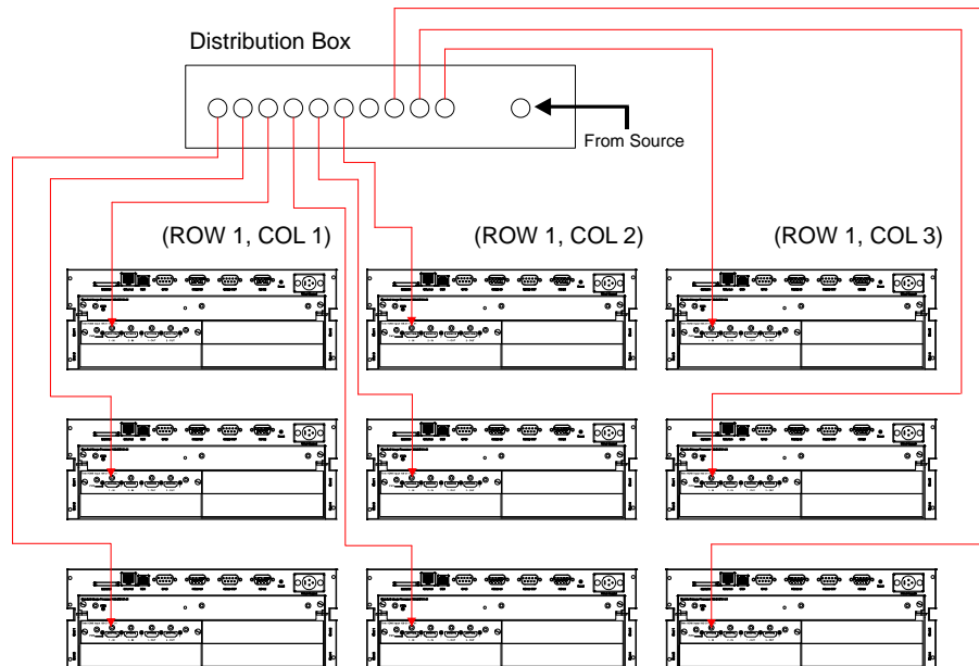
FIGURE 2-27 USE OF DISTRIBUTION BOX
