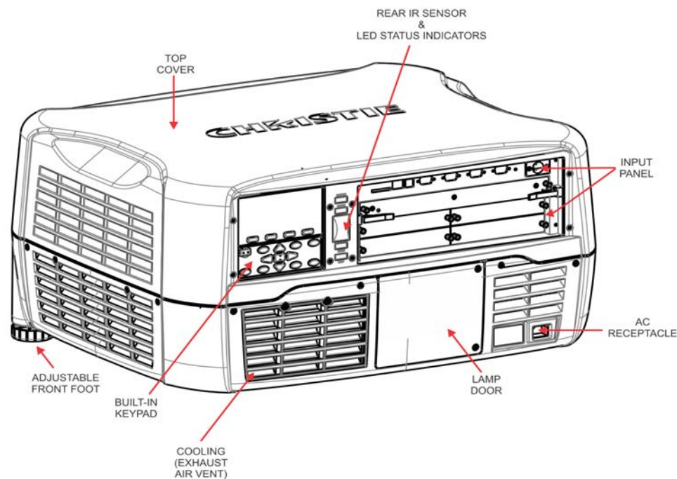
FIGURE 2-5 REAR ORIENTATION
