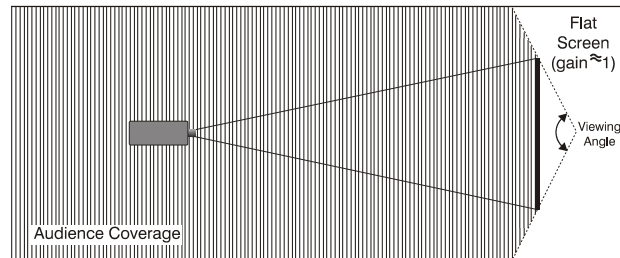
FIGURE 2-9 FLAT SCREEN
