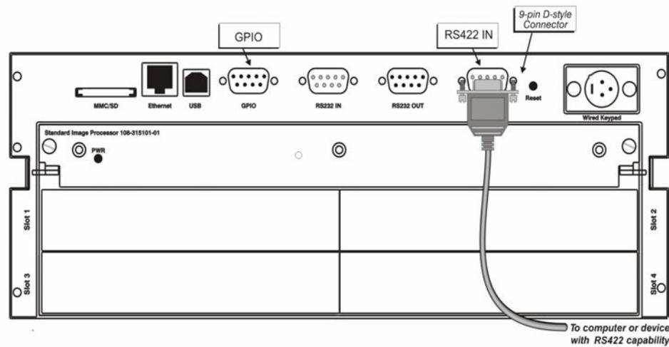
FIGURE 2-21 CONNECTING RS-422
