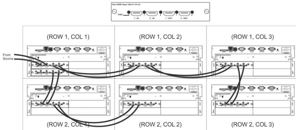
FIGURE 2-31 2X3 SINGLE WIRING LOOP-THROUGH - NO PIP IS SUPPORTED
