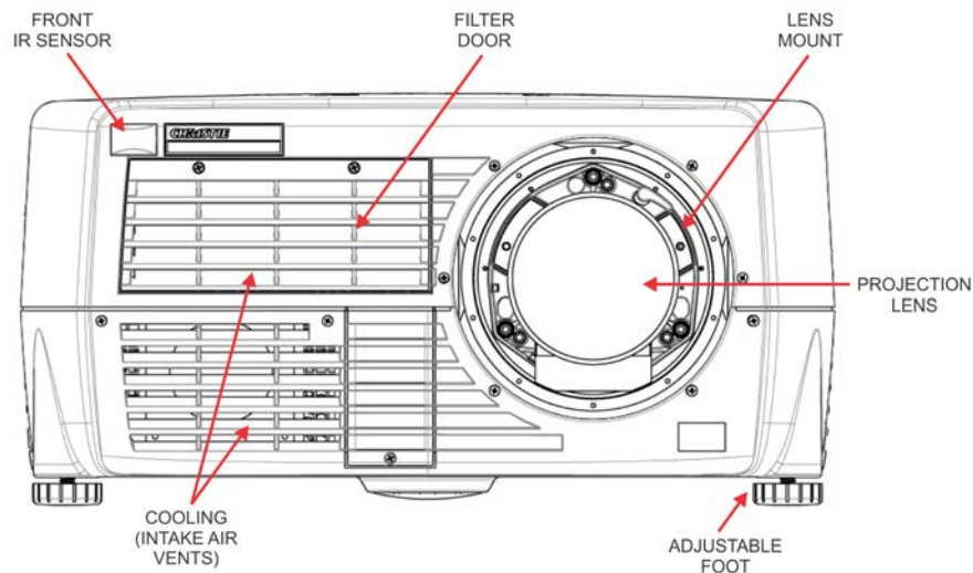
FIGURE 2-8 FRONT ORIENTATION
