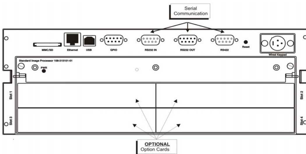
FIGURE 2-26 INPUT PANEL
