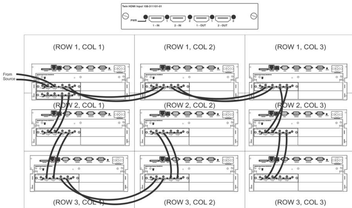
FIGURE 2-32 3X3 LOOP-THROUGH WIRING SOLUTION
