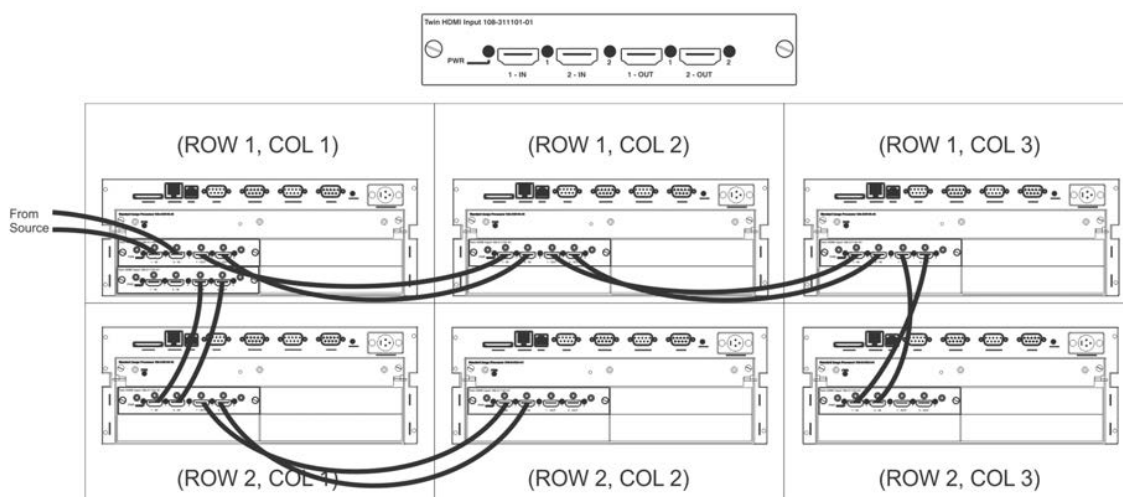
FIGURE 2-30 2x3 LOOP-THROUGH WIRING SOLUTION
