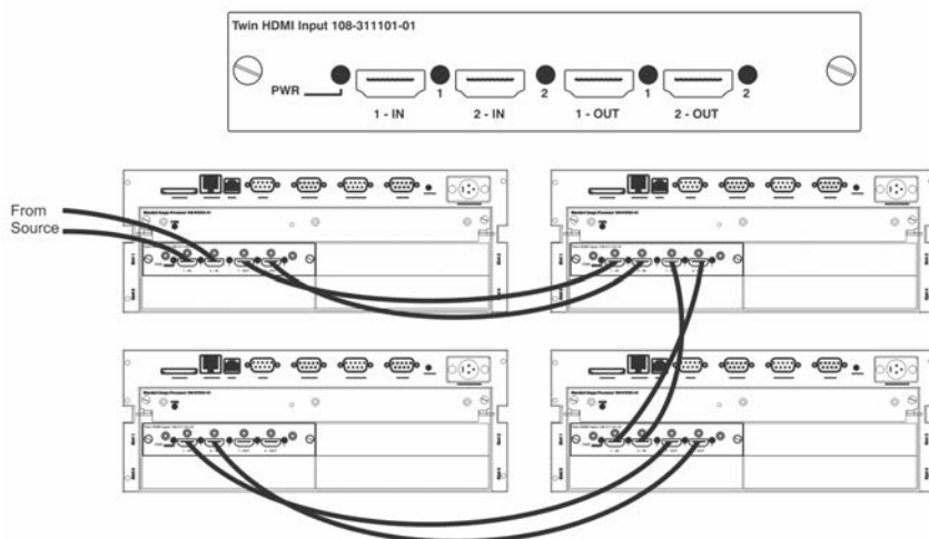
FIGURE 2-29 2x2 WIRING SOLUTION
