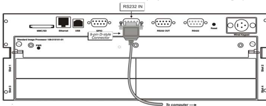
FIGURE 2-20 CONNECTING RS-232
