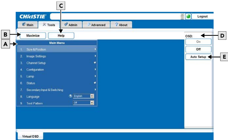
FIGURE 4-6 TOOLS WINDOW
