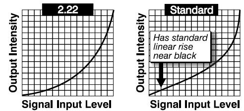
FIGURE 3-29 GAMMA CURVE
