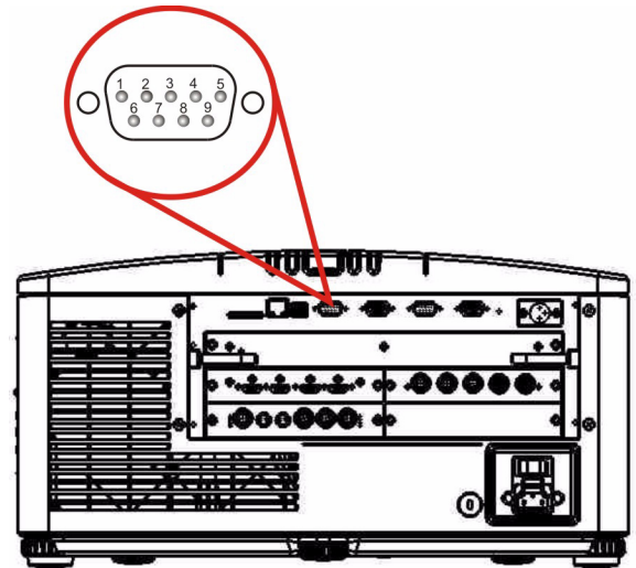
FIGURE B-1 - GPIO CONNECTOR
