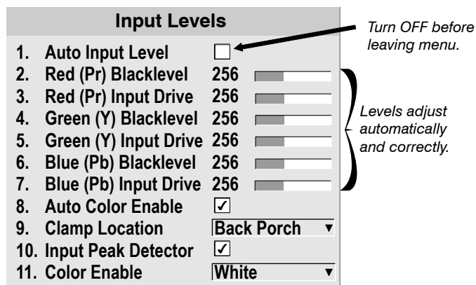
FIGURE 3-28 INPUT LEVELS
