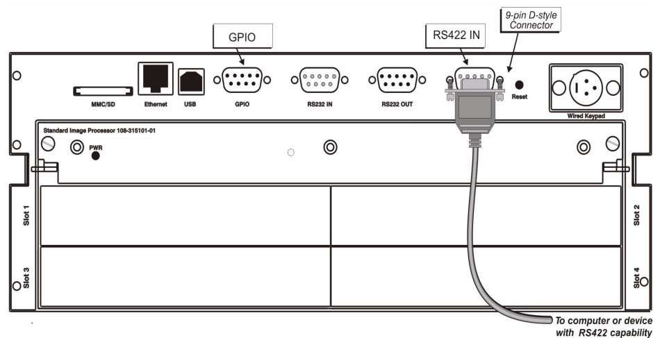
FIGURE 2-20 CONNECTING RS-422
