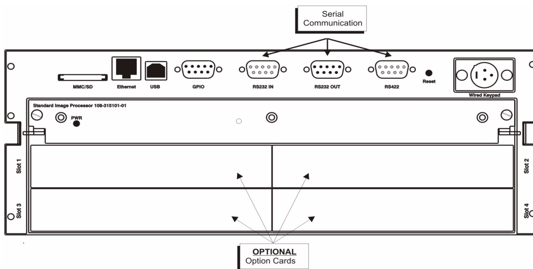
FIGURE 2-25 INPUT PANEL
