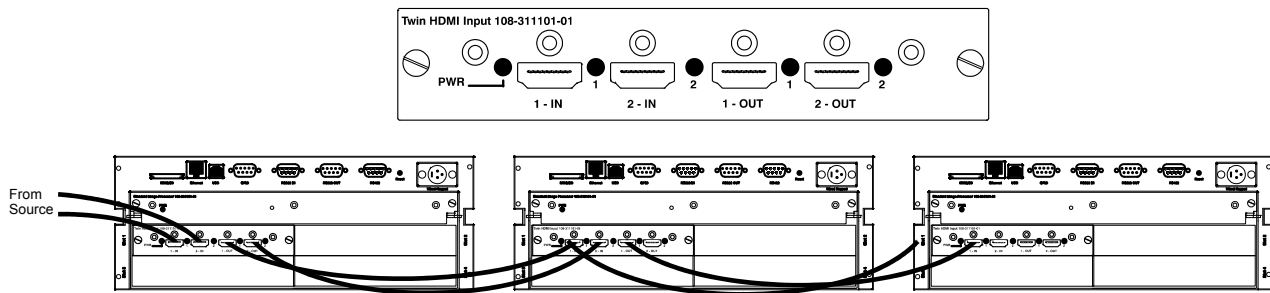
FIGURE 2-27 1x3 WIRING SOLUTION
