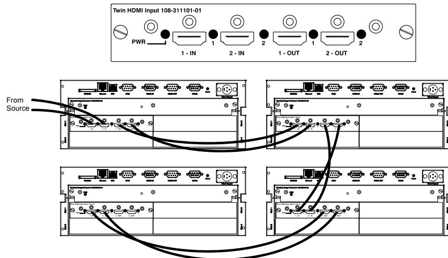
FIGURE 2-28 2x2 WIRING SOLUTION
