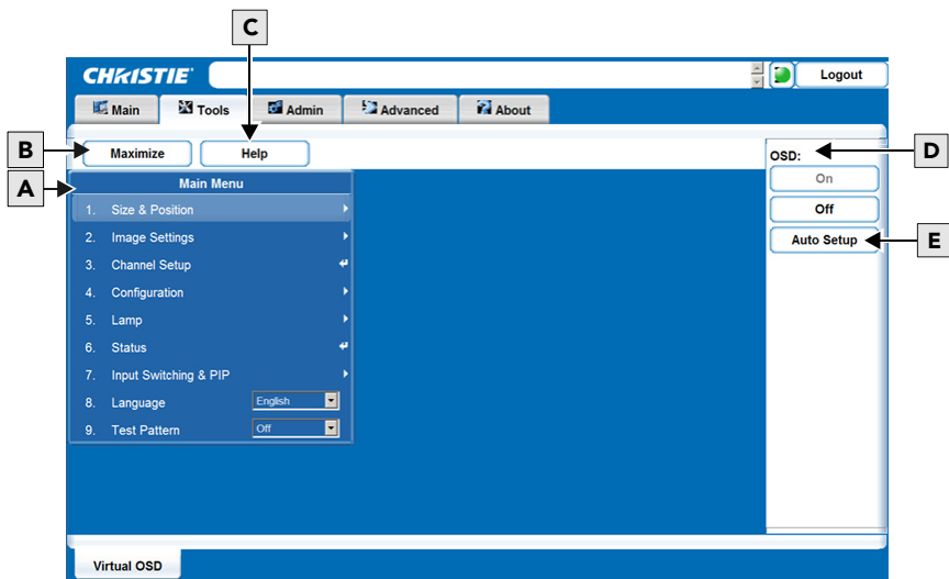
FIGURE 4-6 TOOLS WINDOW
