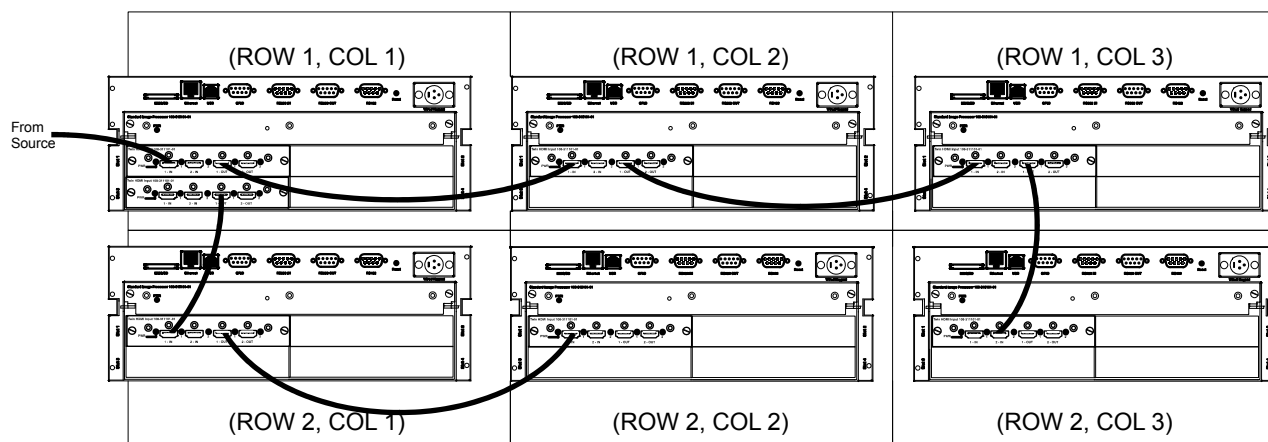
FIGURE 2-30 2X3 SINGLE WIRING LOOP-THROUGH - NO PIP IS SUPPORTED
