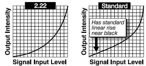
FIGURE 3-30 GAMMA CURVE
