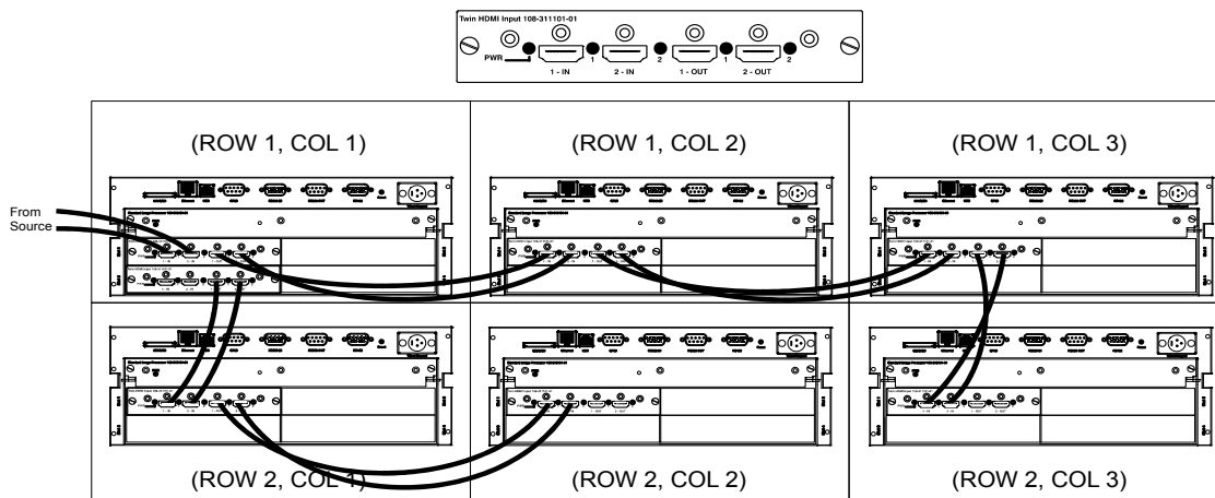
FIGURE 2-29 2x3 LOOP-THROUGH WIRING SOLUTION
