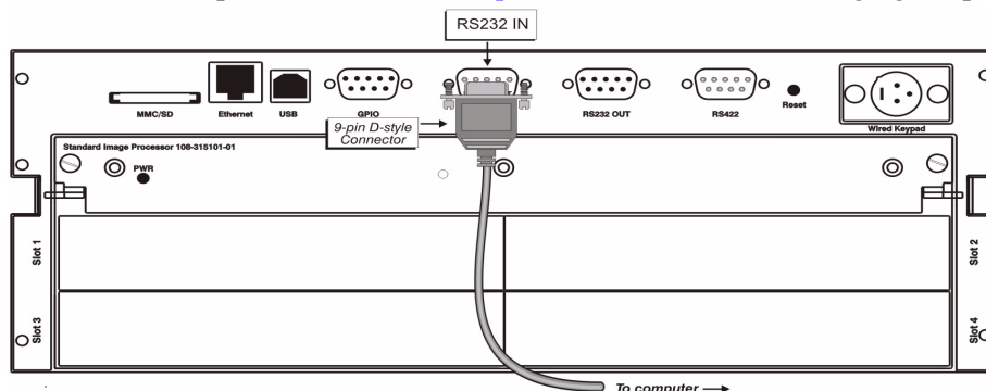
FIGURE 2-19 CONNECTING RS-232
