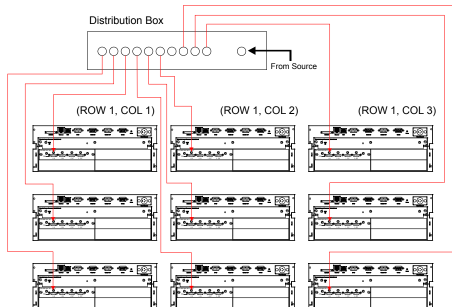
FIGURE 2-26 USE OF DISTRIBUTION BOX
