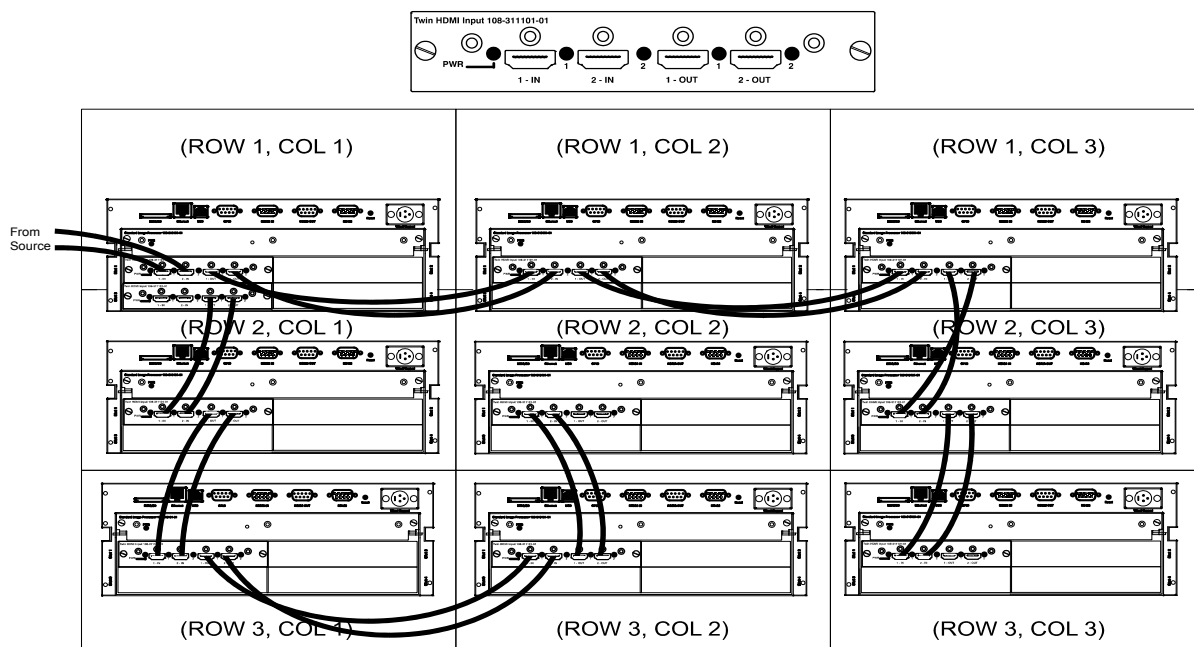
FIGURE 2-31 3X3 LOOP-THROUGH WIRING SOLUTION
