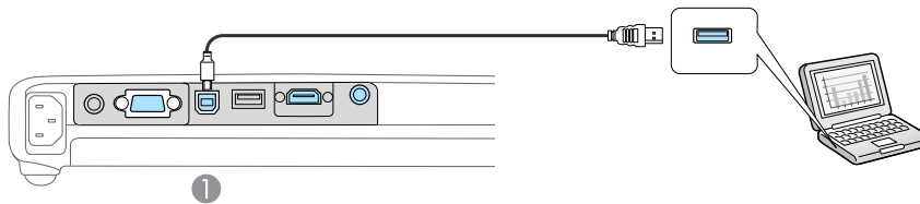
1 USB TypeB port
