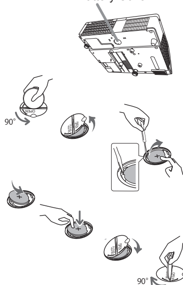
Battery Cover
