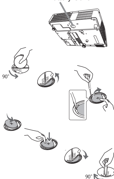
Battery Cover
