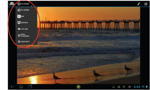
Android screen
