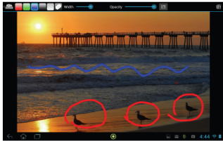
Android screen
