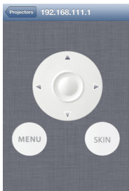
iOS screen
