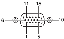
COMPUTER IN/OUT (Mini D-SUB 15-pin)
