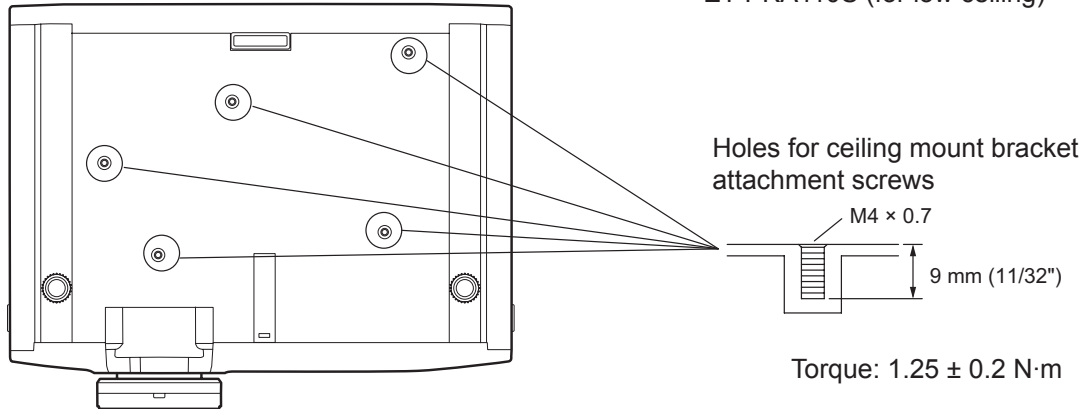
Bottom view
