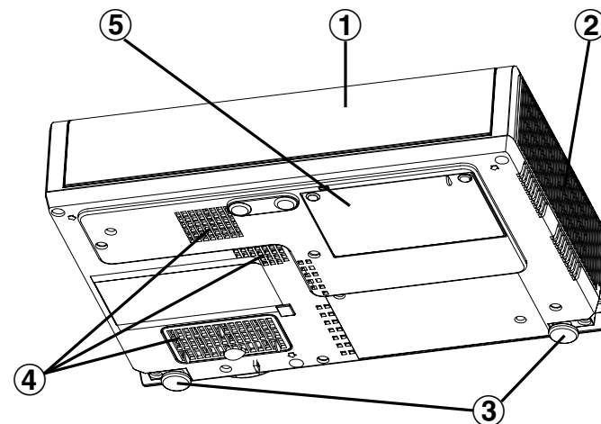
Projector <Back and bottom>
