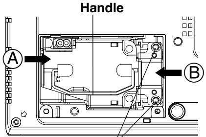
Lamp unit fixing screws
