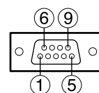
D-Sub 9-pin (female) external appearance
