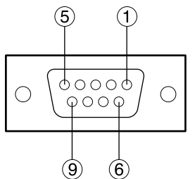
D-Sub 9-pin (female) external appearance
