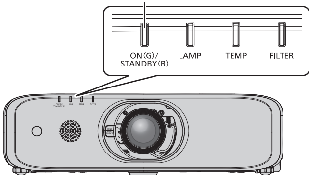
Power indicator <ON (G)/STANDBY(R)>
