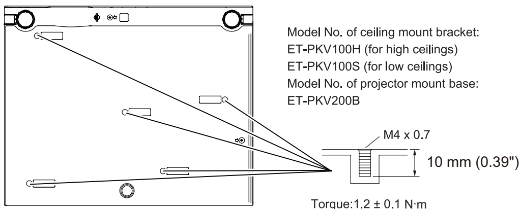
Bottom view
