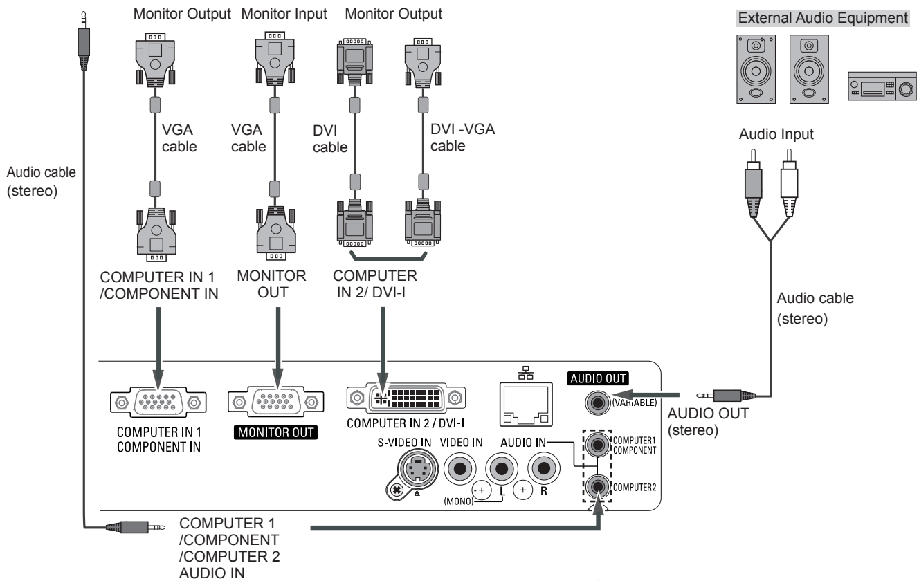
Audio Output
