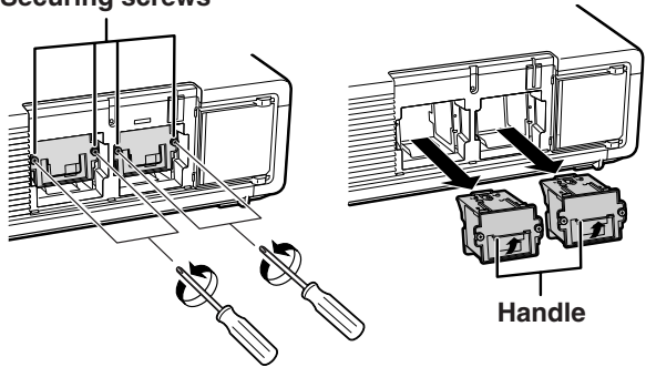
Securing screws
