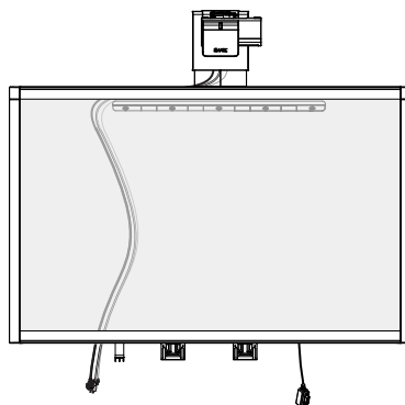
Cable routing for SMART Board 880 interactive whiteboards
