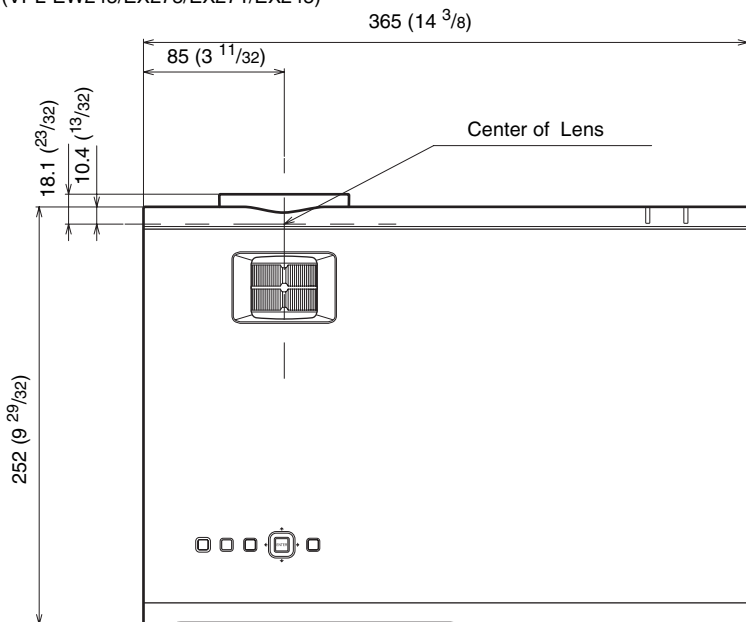
Top (VPL-EW245/EX275/EX271/EX245)
